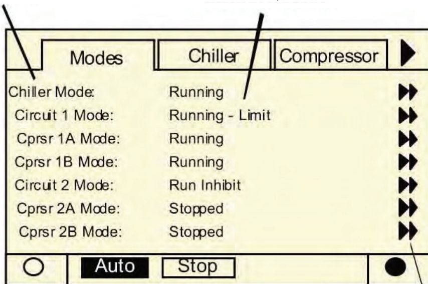
Tela Modes SW Rev 18.0
