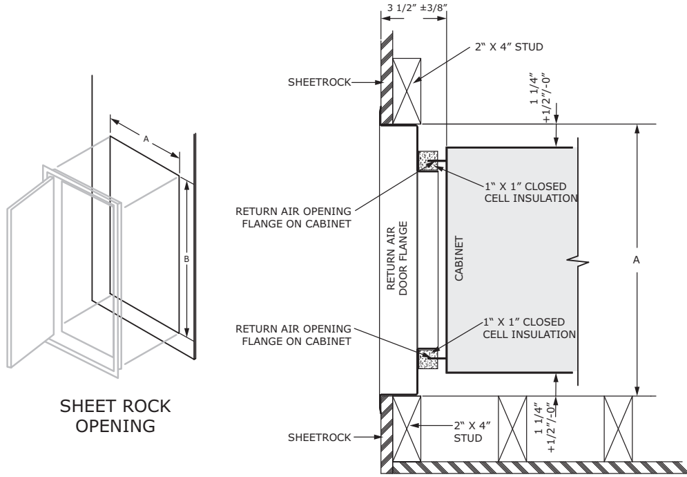
Figure 18. Hinged acoustical door with standard base
